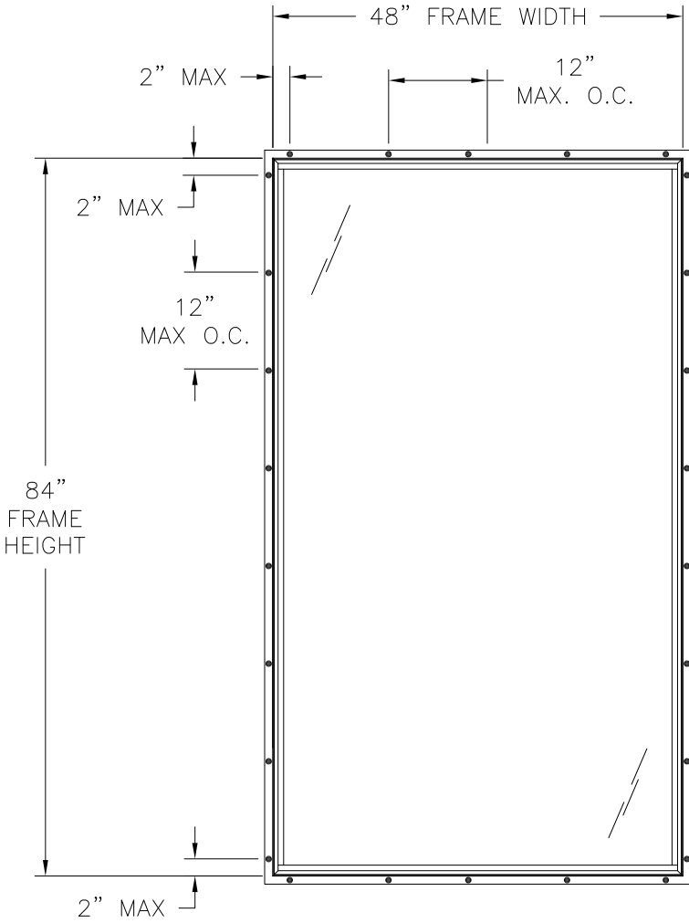
400/475 VINYL PICTURE WINDOW EXTERIOR VIEW
